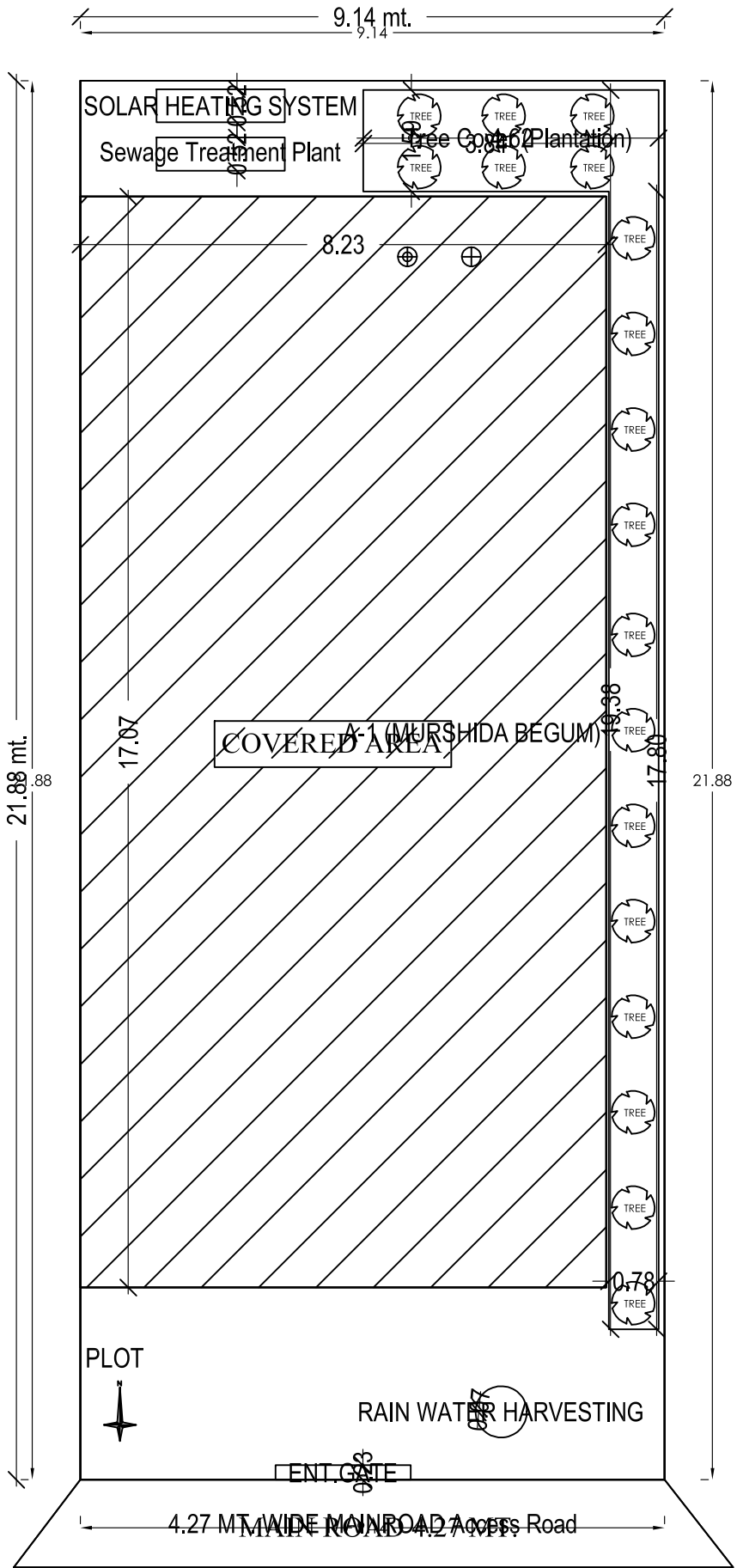
SITE PLAN
