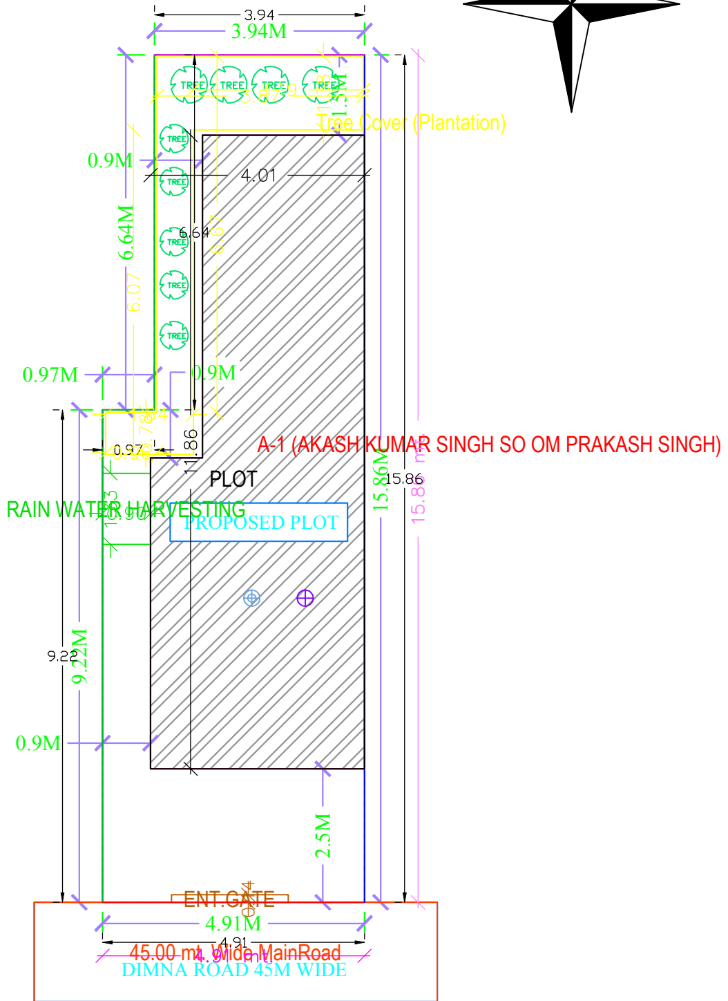
SITE PLAN
