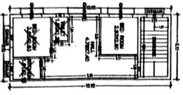
FIRST FLOOR PLAN (Proposed) (SCALE 1:100)
