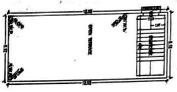
TERRACE FLOOR PLAN (SCALE 1:100)
