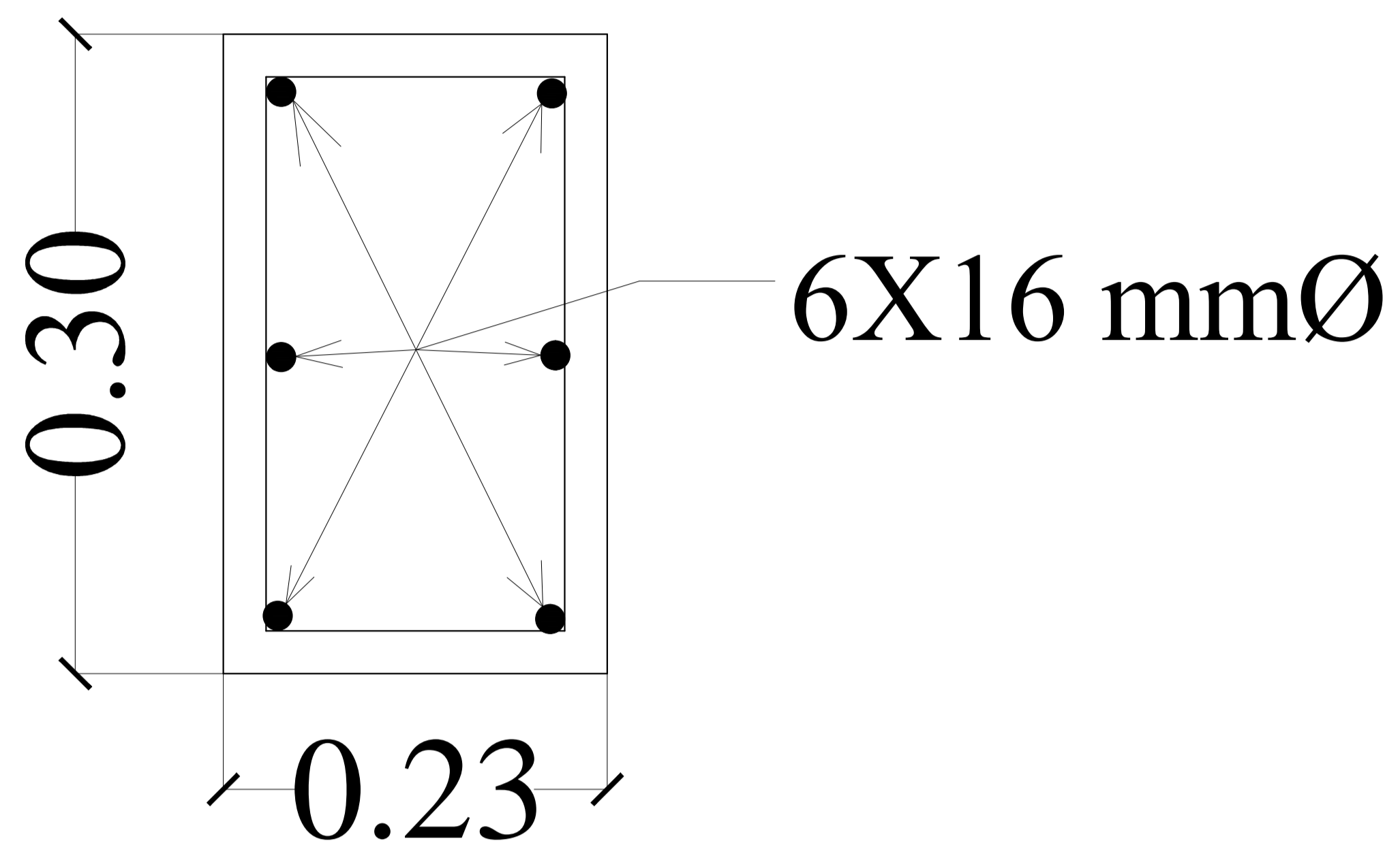
SECTION OF COLUMN
