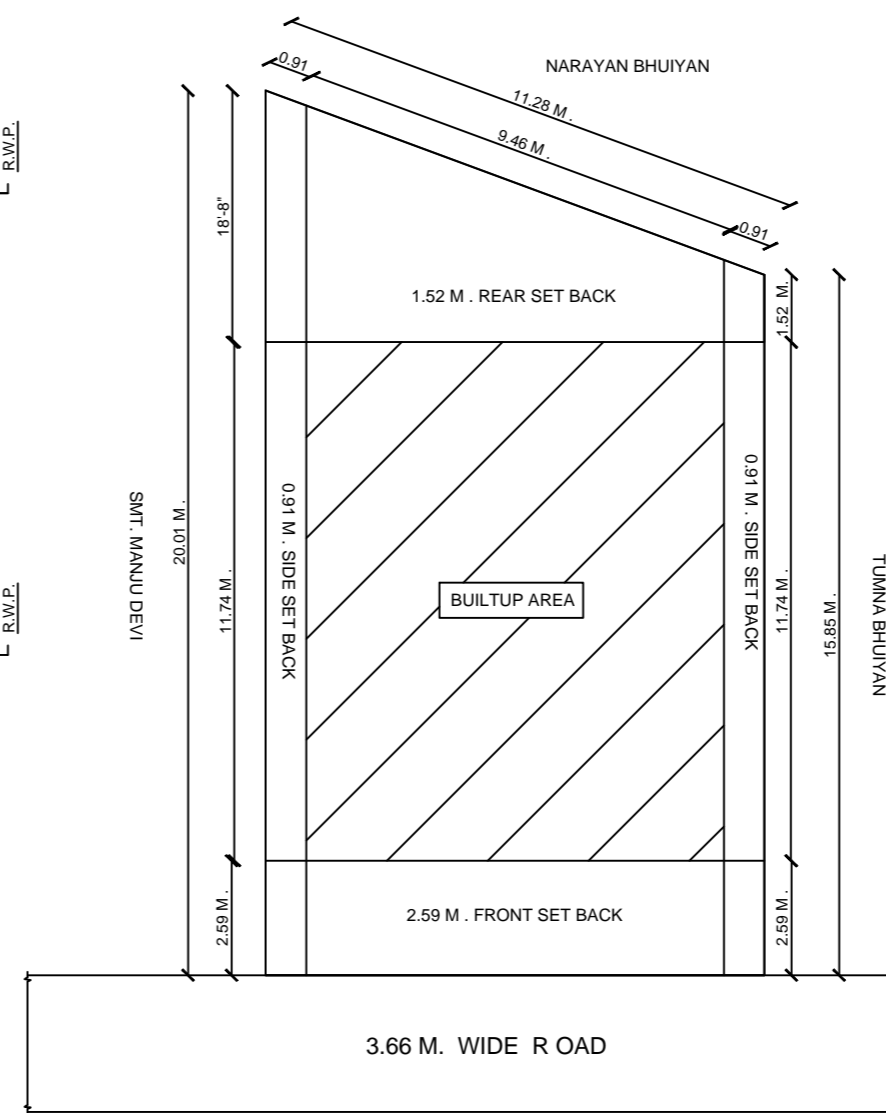
SITE PLAN
