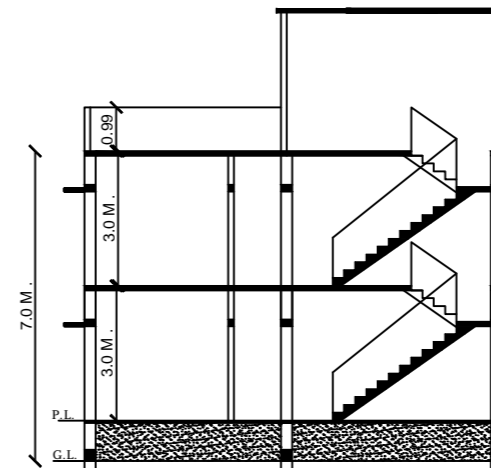
SECTION- xx
