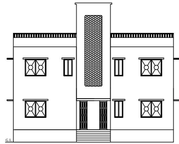
NORTH SIDE ELEVATION
