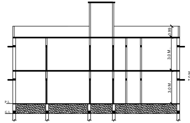
SECTION-YY
