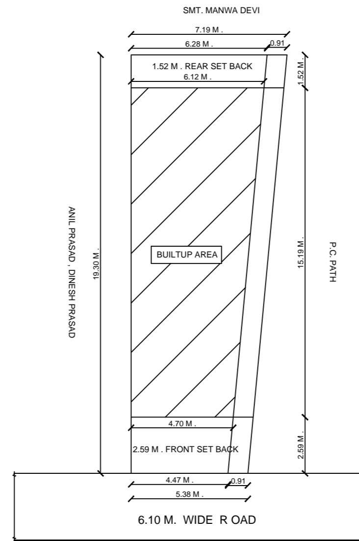
SITE PLAN
