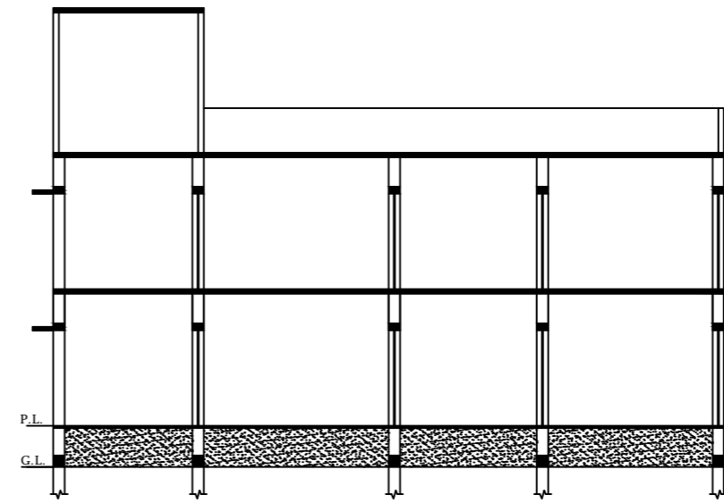
SECTION-YY
