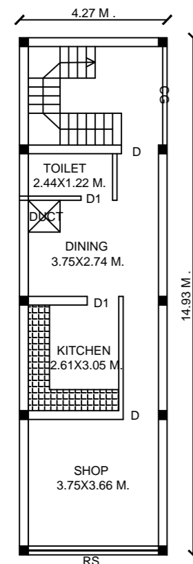
PROPOSED GROUND FLOOR PLAN
