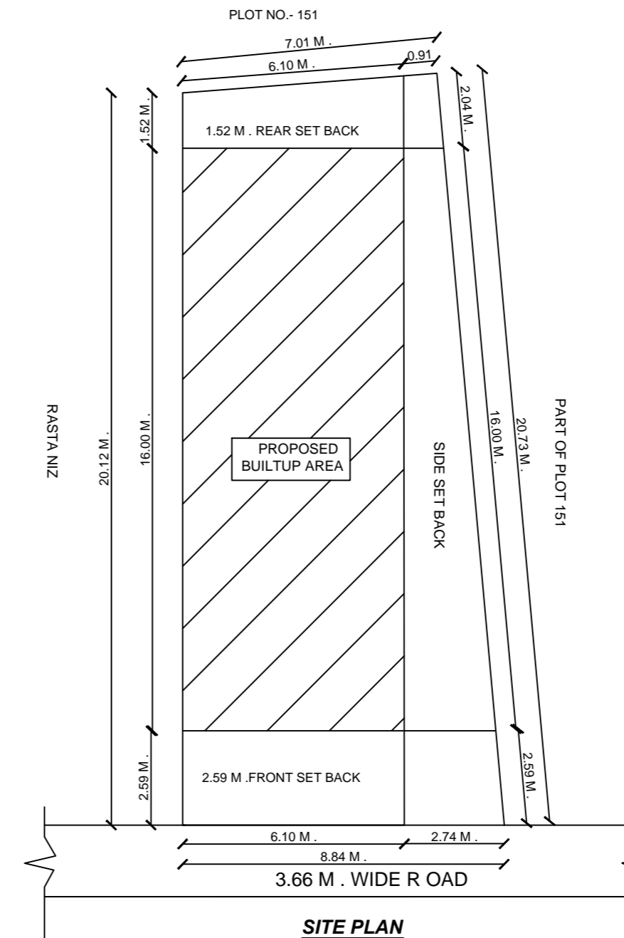
SITE PLAN
