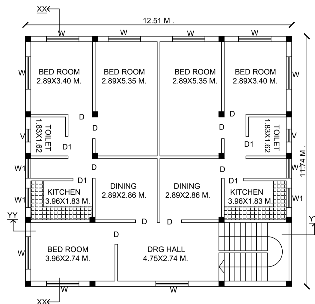
PROPOSED FIRST & SECOND FLOOR PLAN
