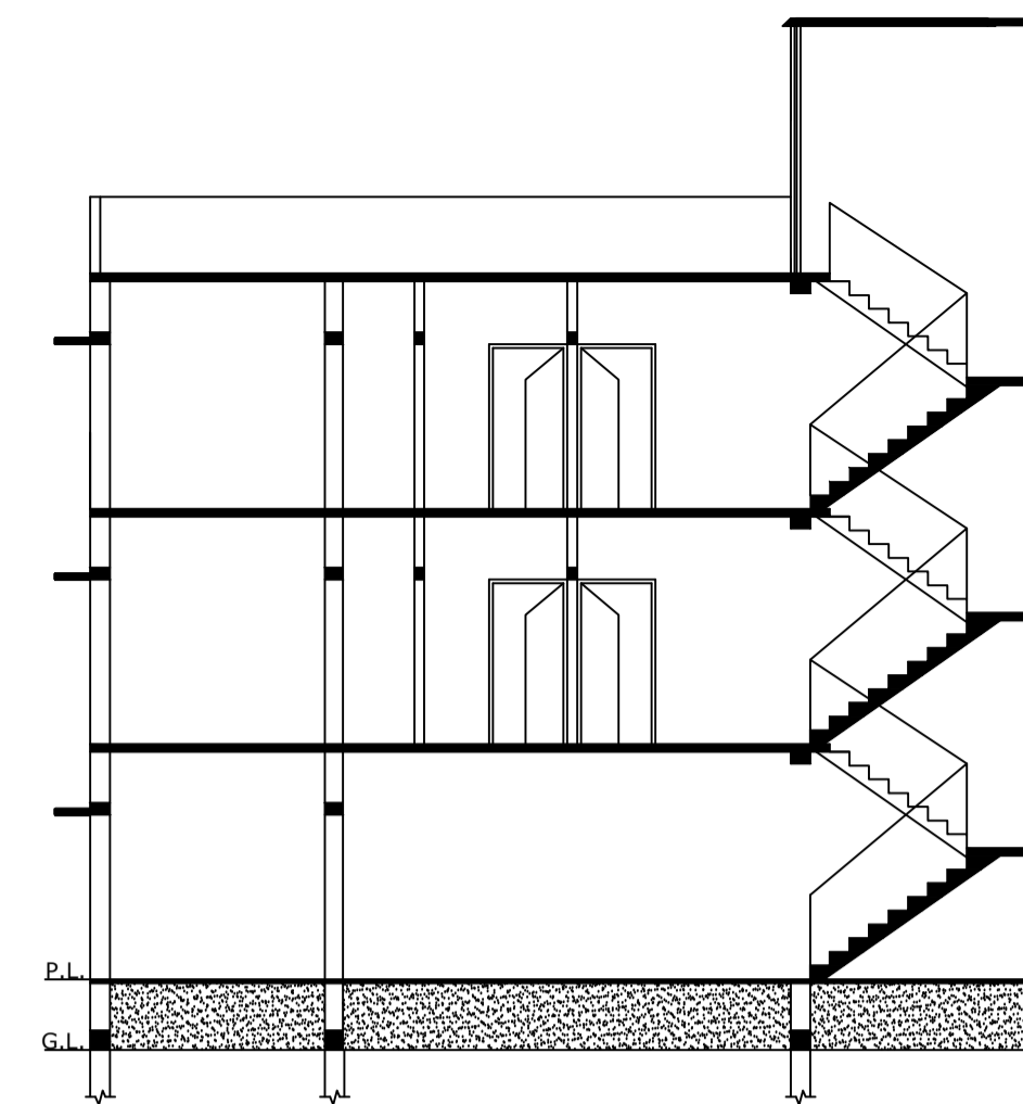
SECTION-YY
