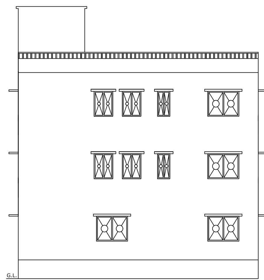
NORTH SIDE ELEVATION
