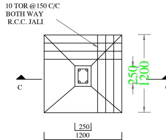
PLAN DETAIL OF FOUNDATION
