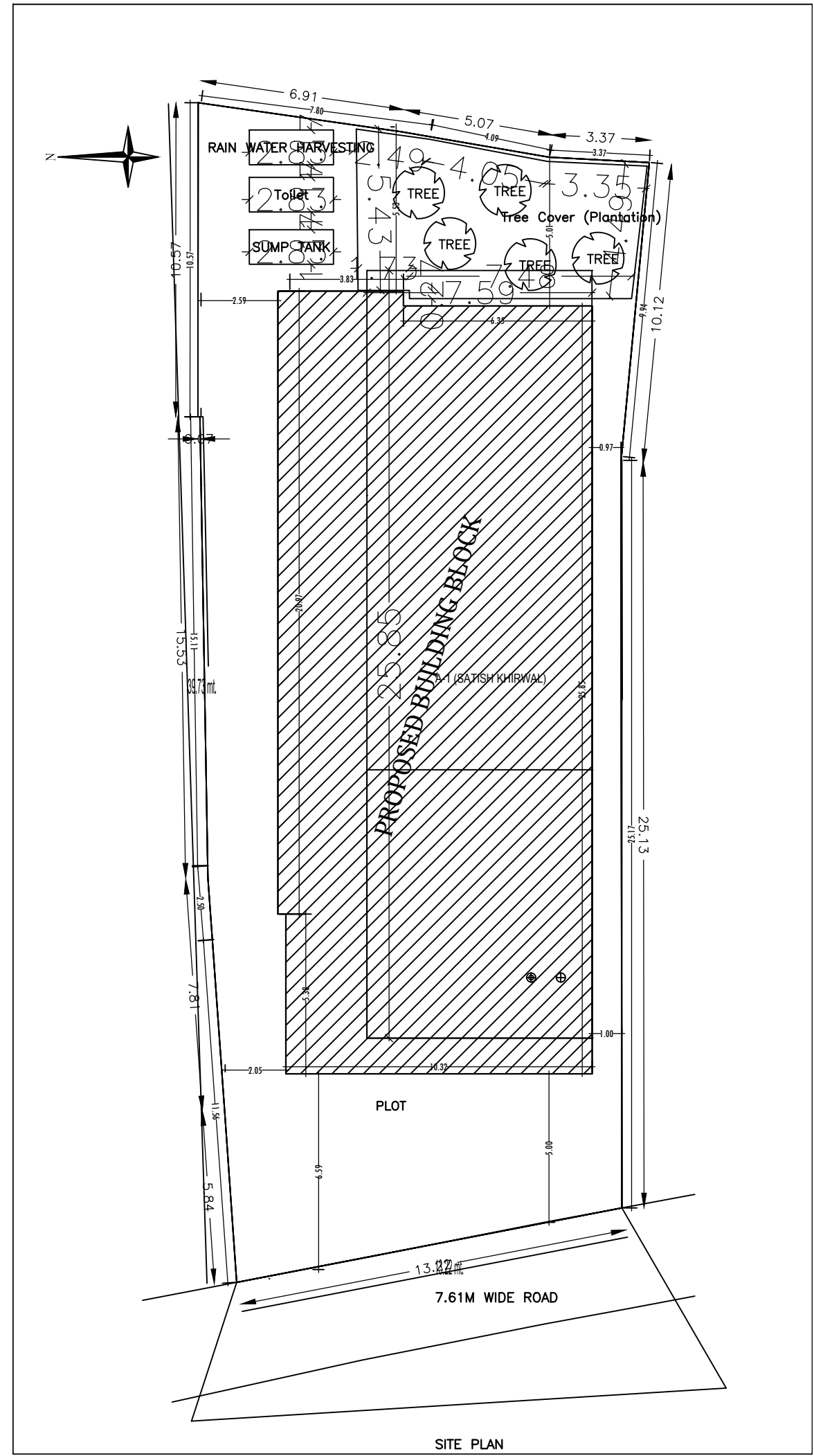
SITE PLAN
