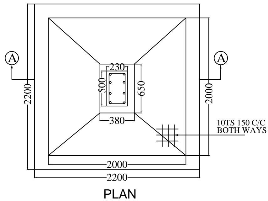
FOOTING PLAN (AS/STRL. DESIGN) SCALE N.T.S
