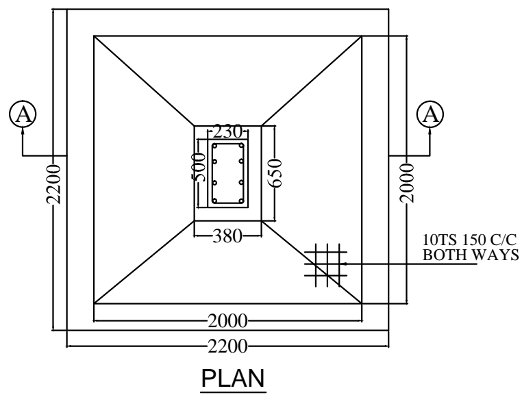
PLAN FOOTING PLAN (AS/STRL. DESIGN) SCALE N.T.S
