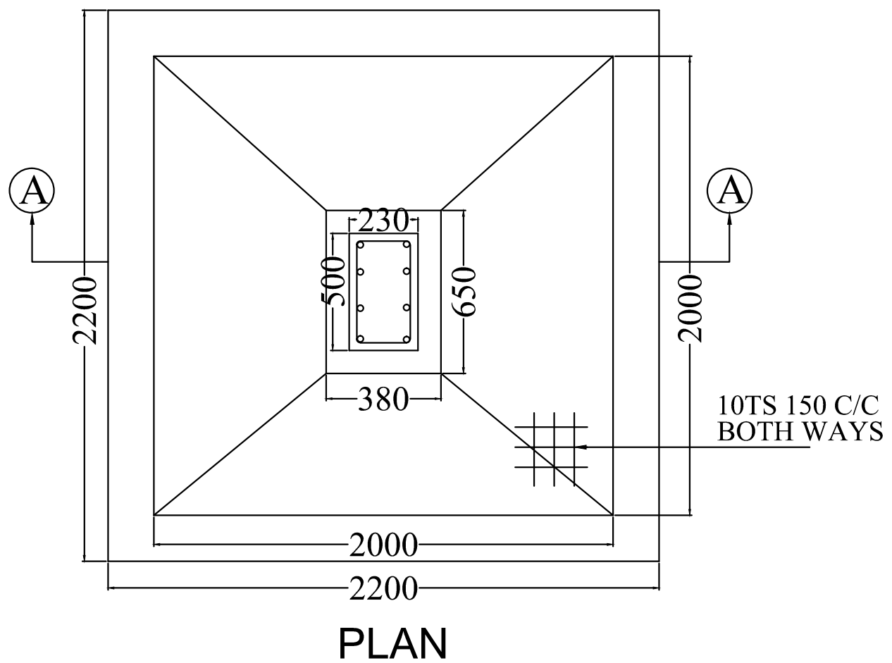
FOOTING PLAN (AS/STRL. DESIGN) SCALE N.T.S
