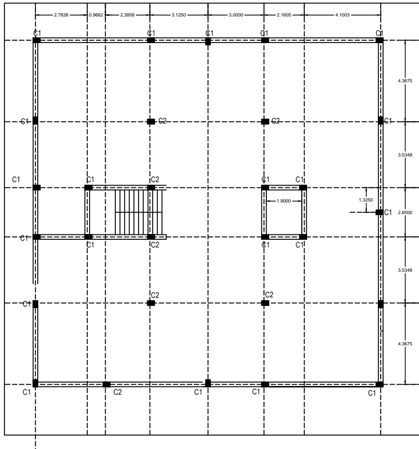
LAY OUT PLAN
