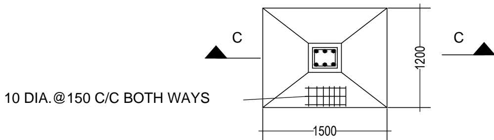
DETAIL OF R.C.C. COLUMN
