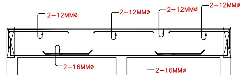
DETAILS OF PLINTH BEAM (250X450)
