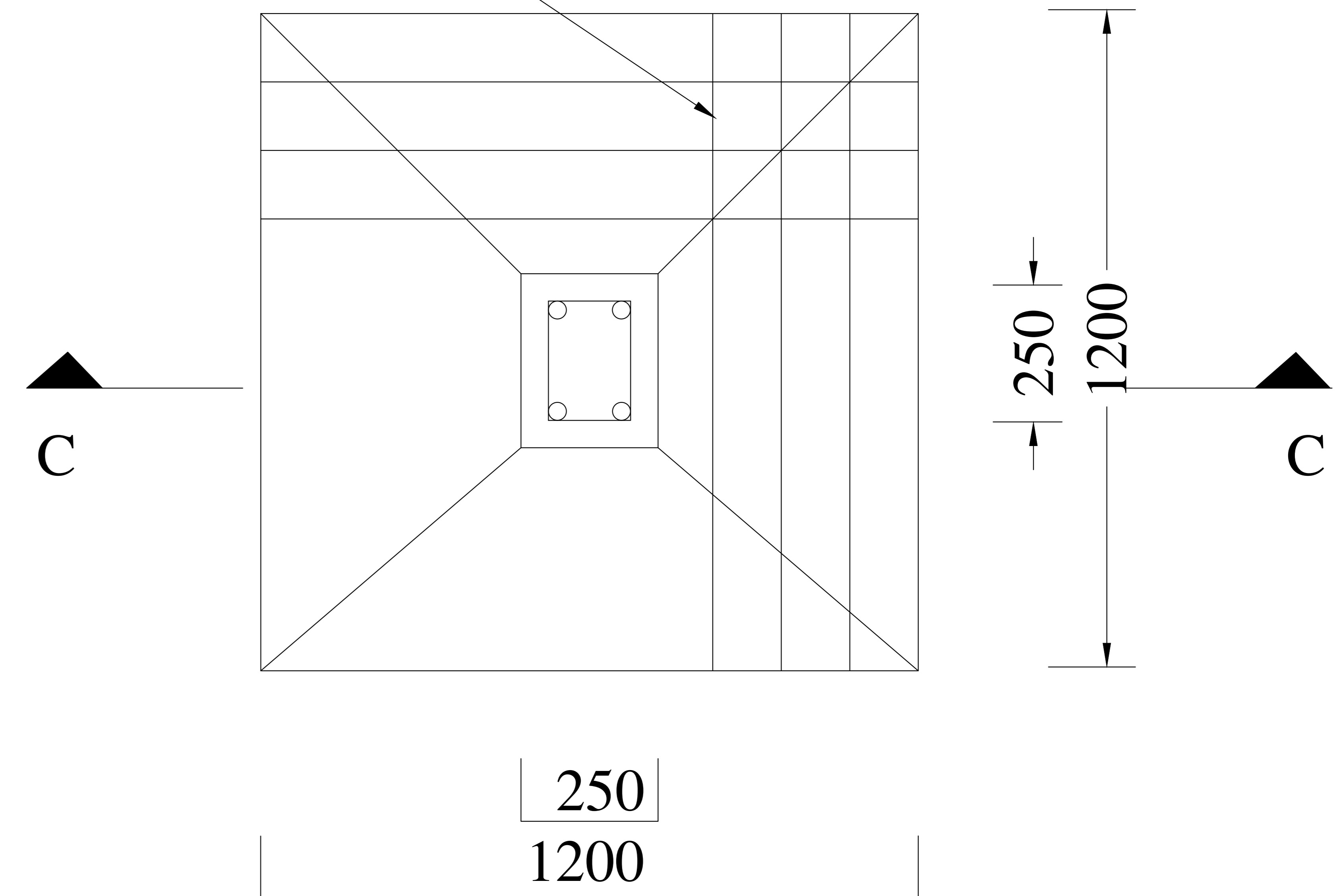
PLAN DETAIL OF FOUNDATION
