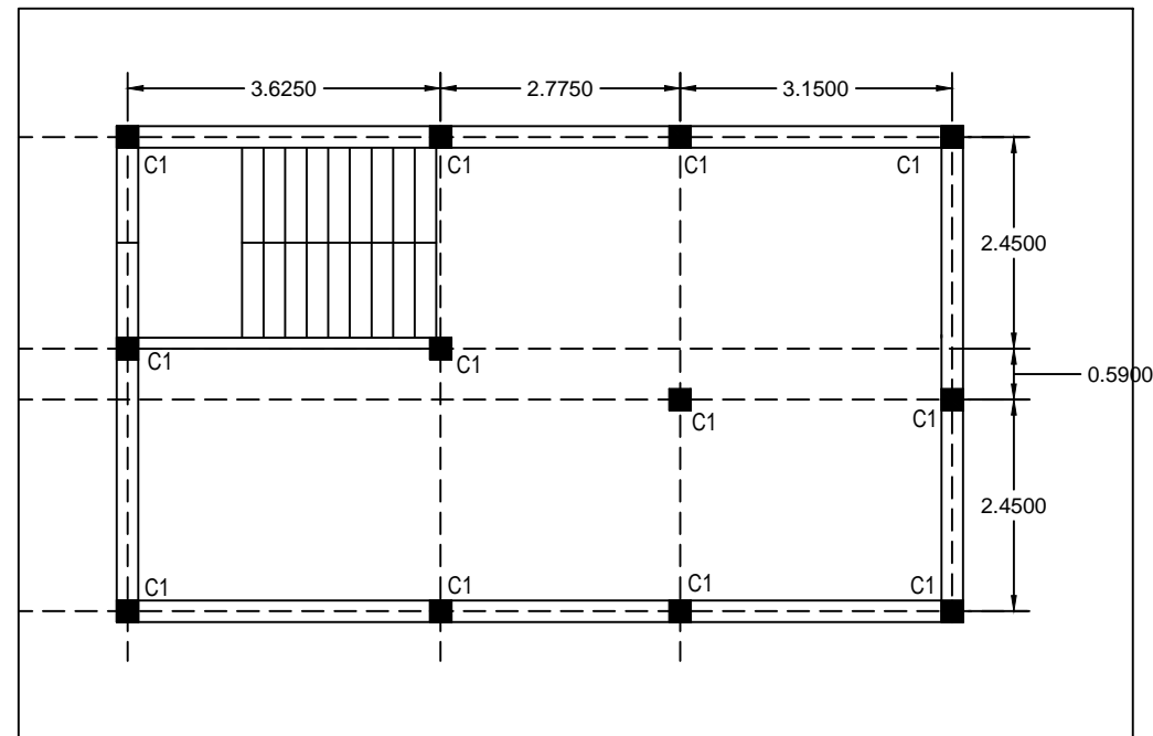
LAY OUT PLAN
