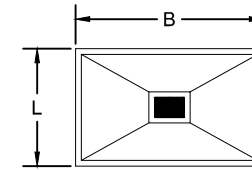
DETAIL OF COL & FOOTING ISOLATED FOOTING
