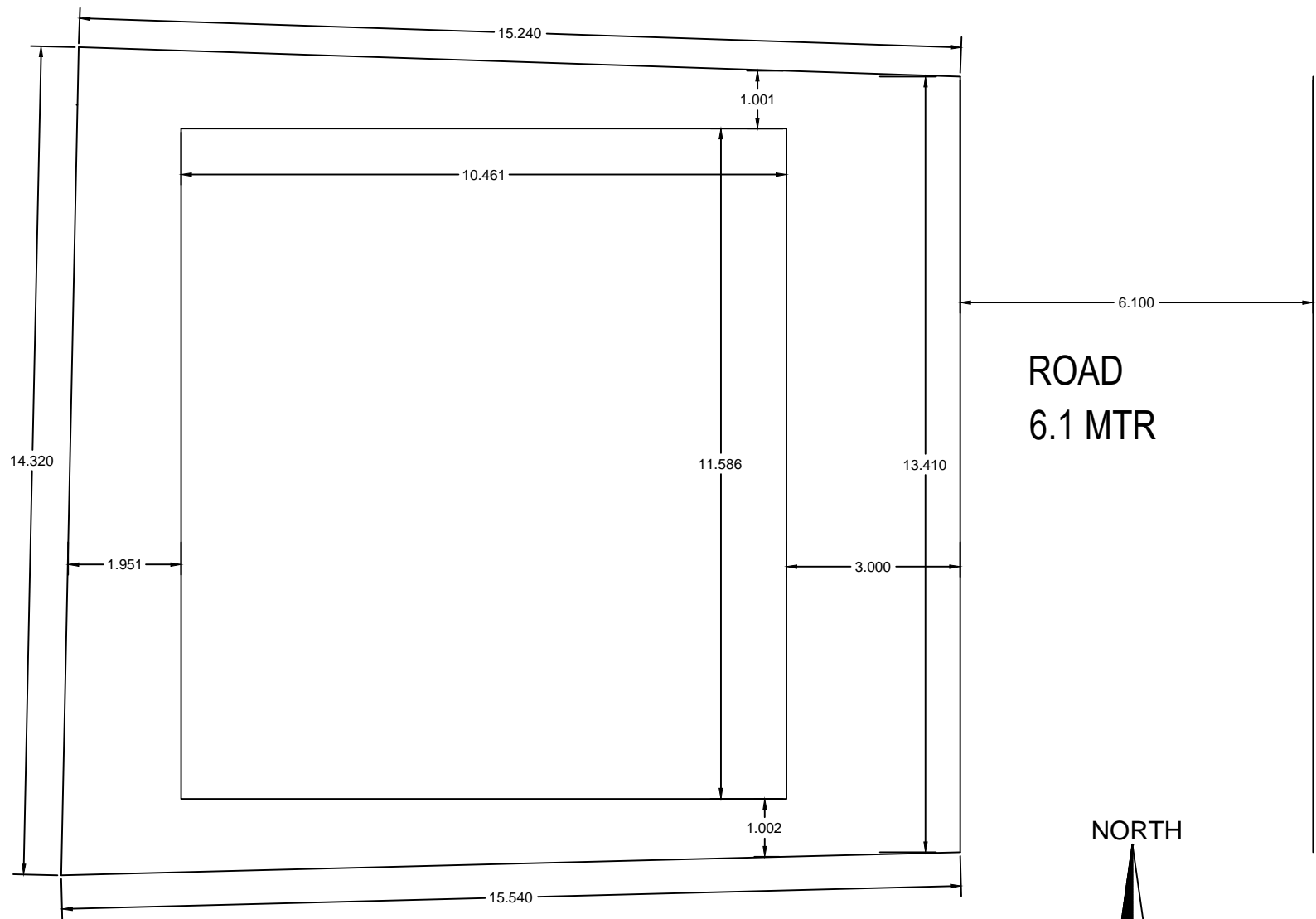
SITE PLAN
