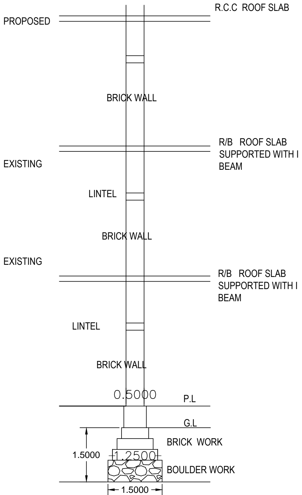
EXISTING FOUNDATION DETAIL
