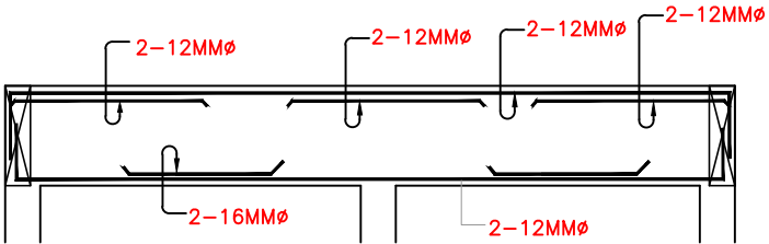
DETAILS OF PLINTH BEAM (250X375)
