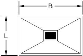
DETAIL OF COL & FOOTING ISOLATED FOOTING
