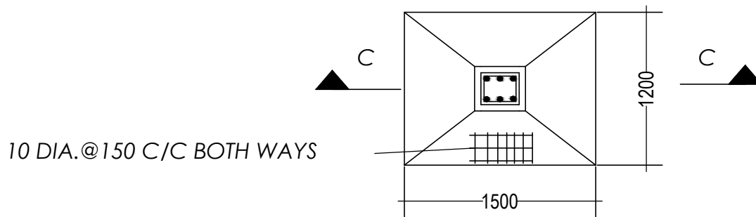
DETAIL OF R.C.C. COLUMN SCALE - 1 : 50
