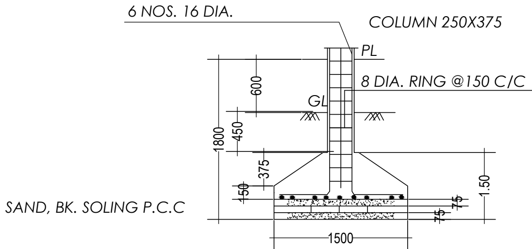
SECTION ON C-C SCALE - 1 : 50
