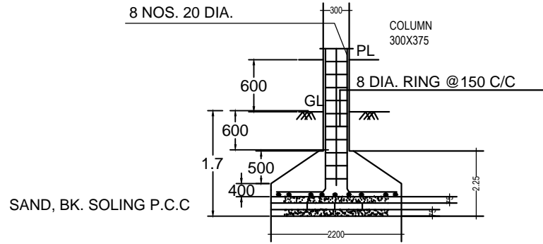
SECTION ON C-C SCALE - 1 : 50
