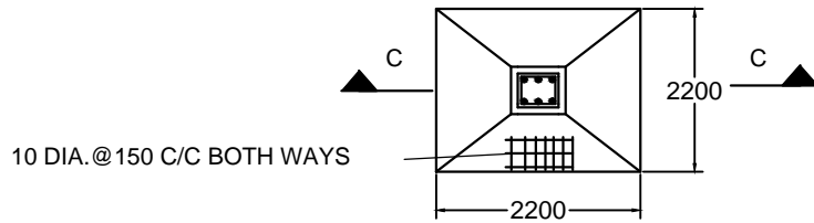
DETAIL OF R.C.C. COLUMN SCALE - 1 : 50
