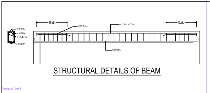
Structure Detail
