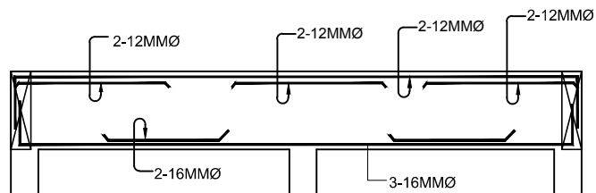
DETAILS OF PLINTH BEAM (250X375)
