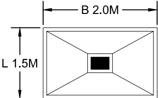
DETAIL OF COL & FOOTING ISOLATED FOOTING
