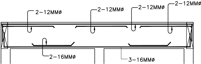
DETAILS OF PLINTH BEAM (250X375)
