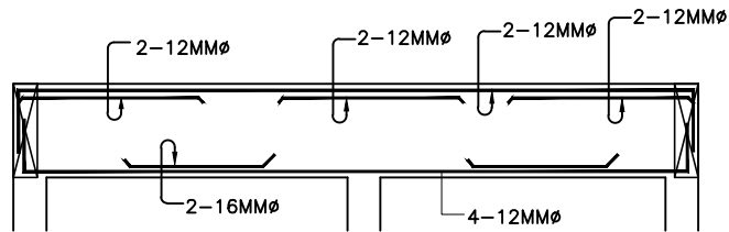
DETAILS OF PLINTH BEAM (250X380)
