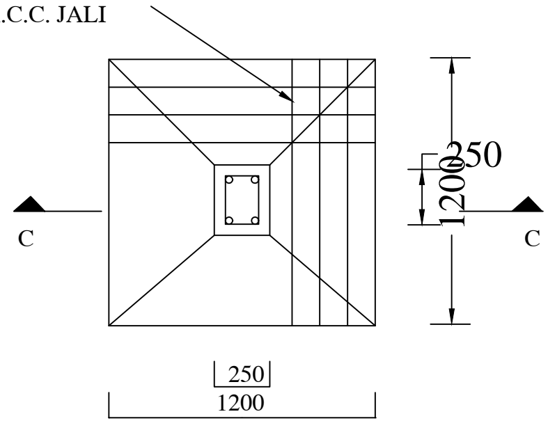
PLAN DETAIL OF FOUNDATION
