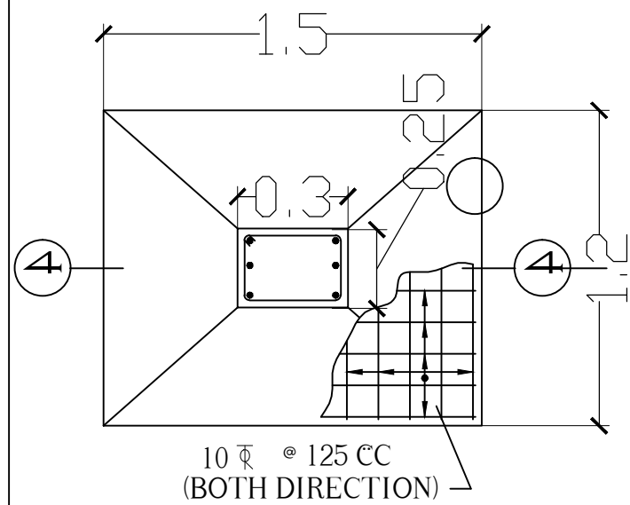
FOUNDATION PLAN OF COLUMN
