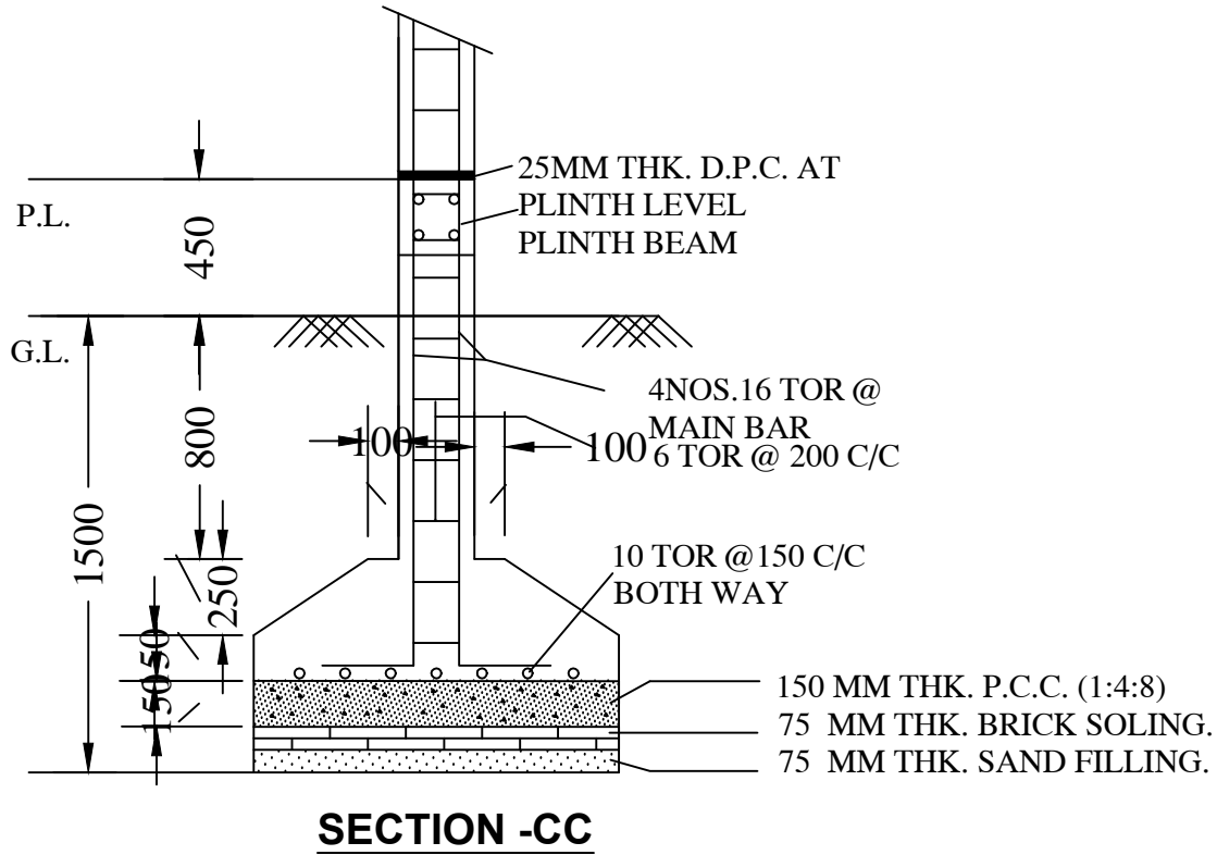
Structure Detail
