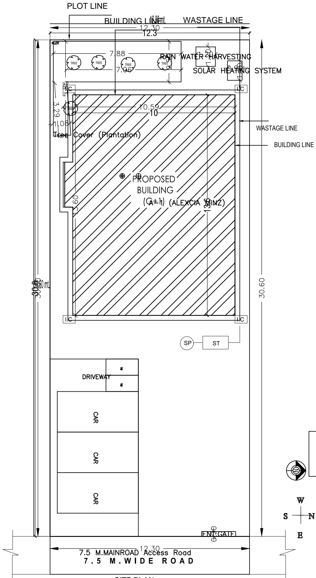
Site plan
