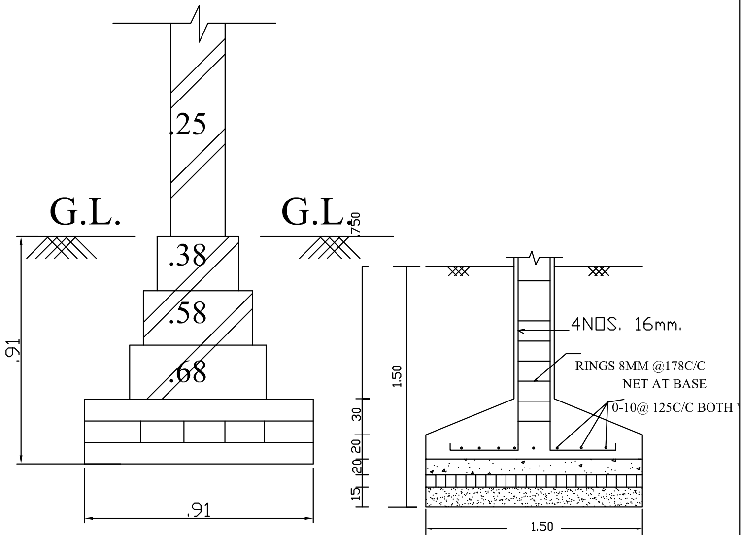
DETAIL OF WALL FOUNDATION (SCALE 1:50)
