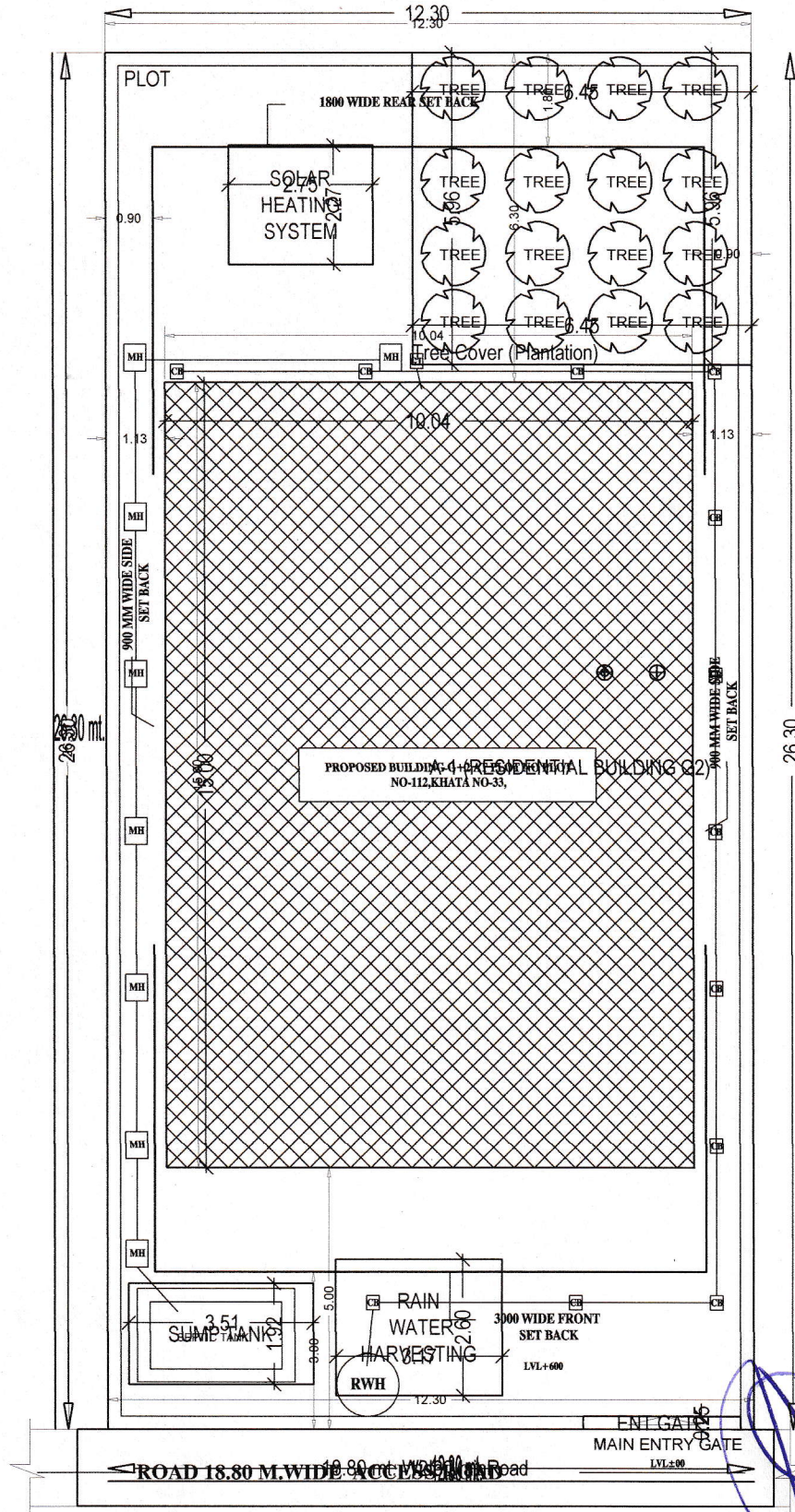
SITE PLAN & DRAINAGE PLAN
