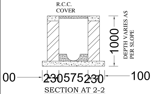
STRUCTURE DETAIL
