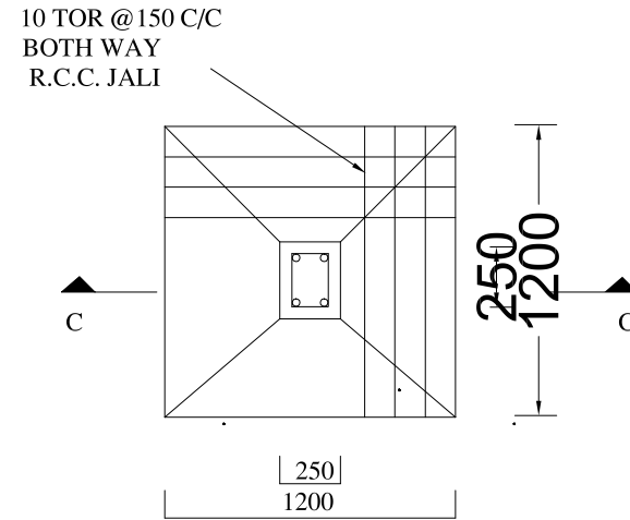
PLAN DETAIL OF FOUNDATION
