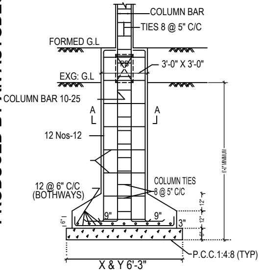
R.C.C. COLUMN & FOOTING DETAIL
