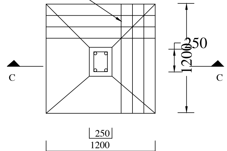
PLAN DETAIL OF FOUNDATION
