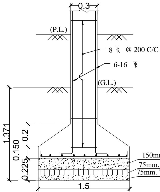
DET. OF FOUND.
