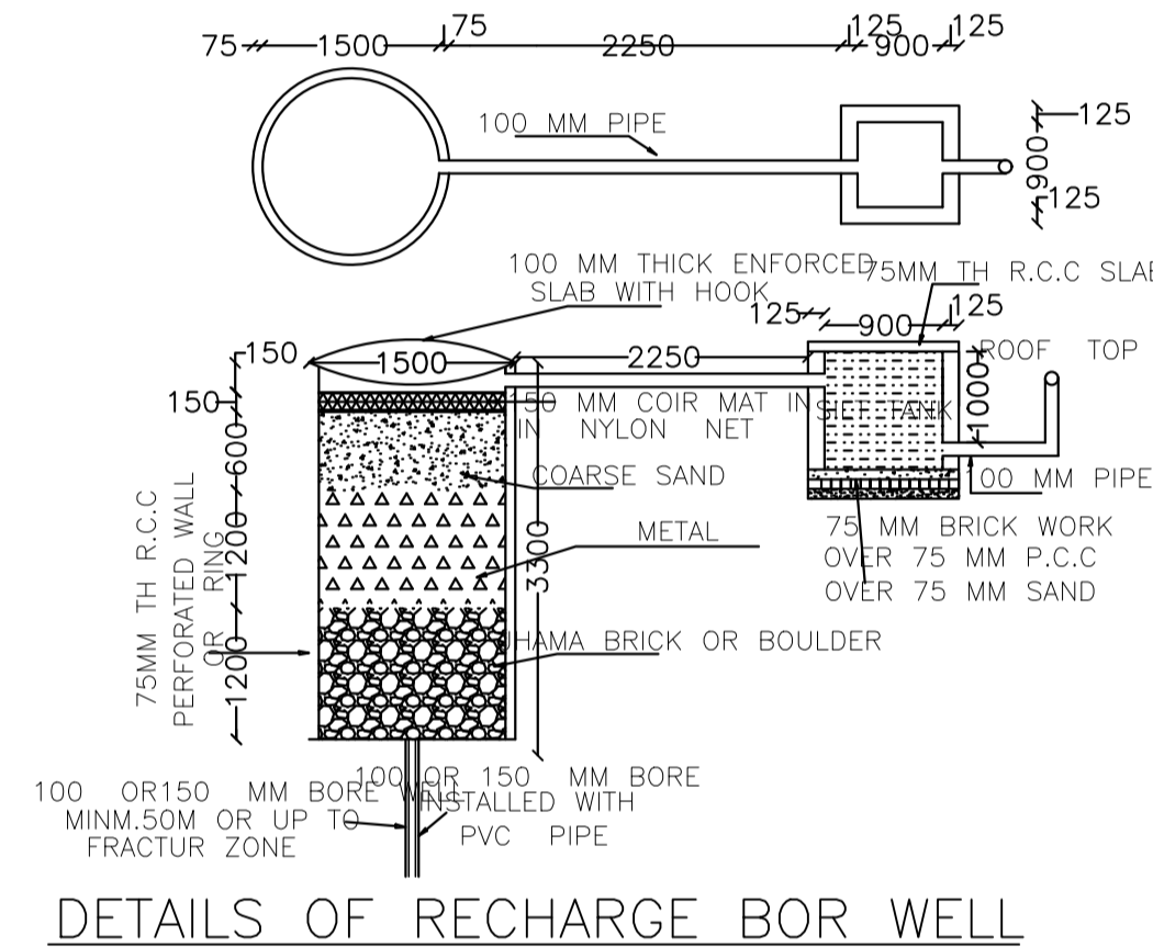
DETAILS OF RECHARGE BOR WELL
