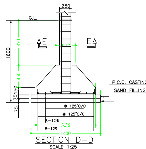
SECTION D-D SCALE 1:25
