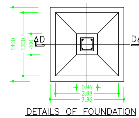
DETAILS OF FOUNDATION SCALE 1:25
