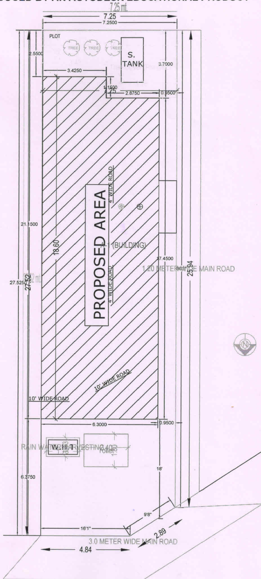
LOCATION PLAN (SCALE -1"=8')
