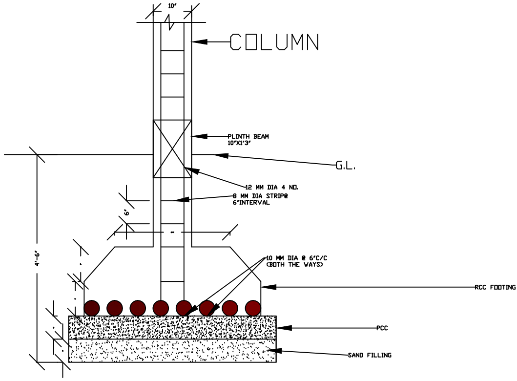
R.C.C. COLUMN DETAIL
