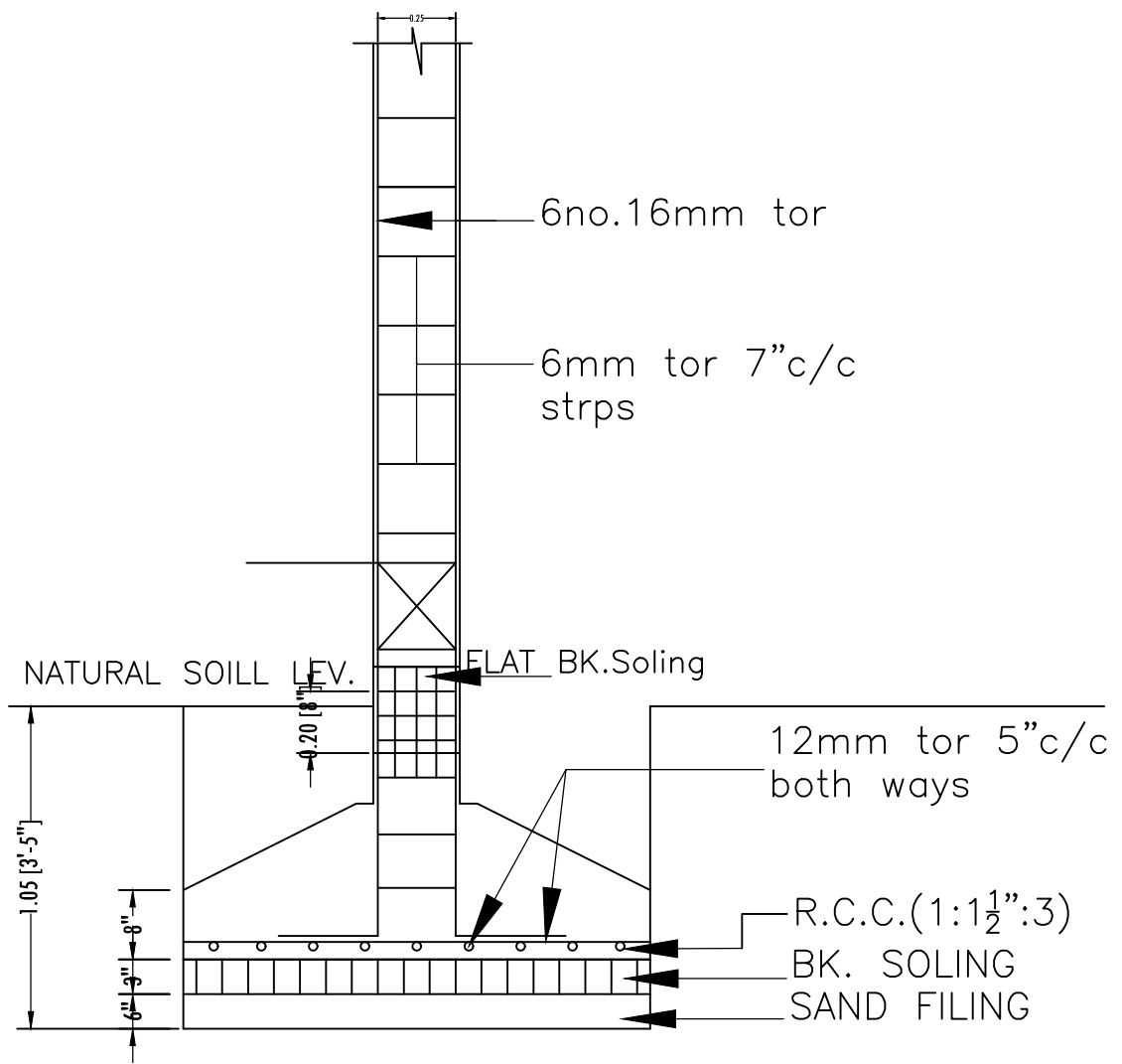
SEC. X-Y R.C.C. COLUMN FDN.DETAIL
