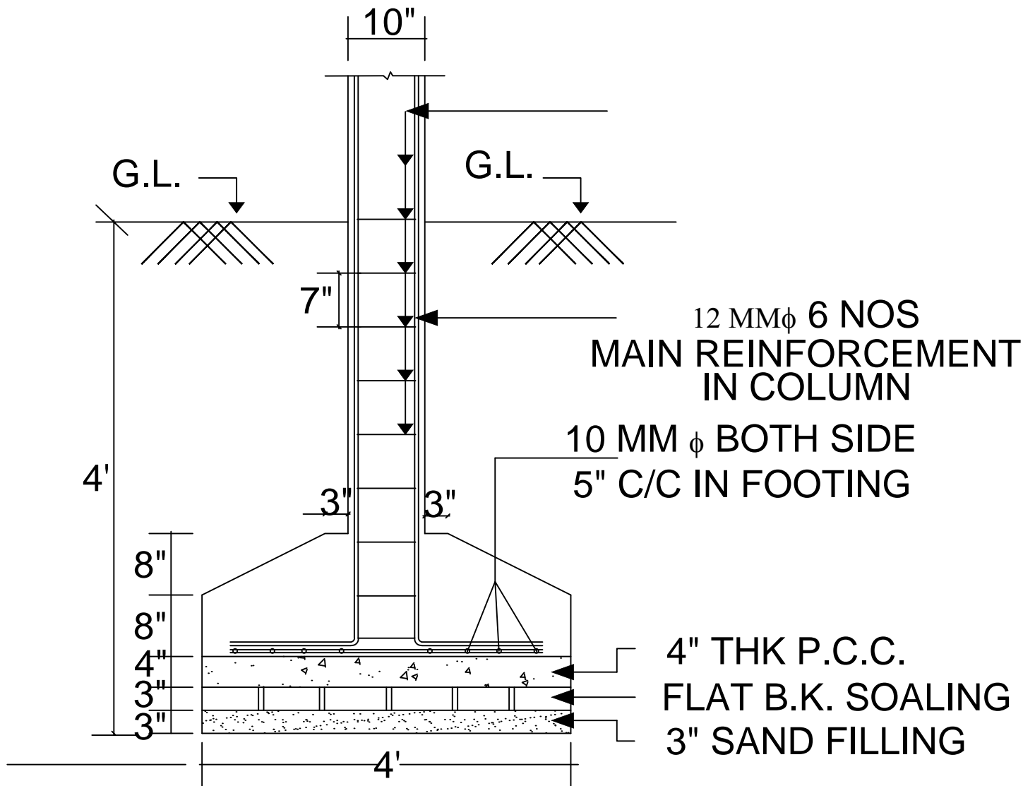
R.C.C. COLUMN FDN. DETAIL, SCALE 1" = 2'-0"
