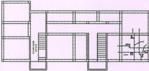
R.C.C. DETAIL FOR GROUND FLOOR & FIRST FLOOR SLAB.
