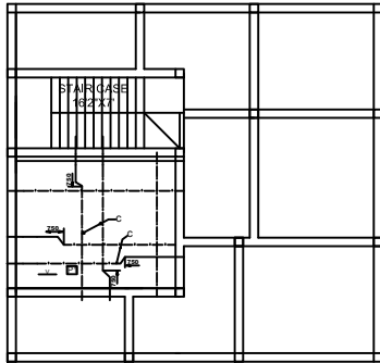
R.C.C. DETAIL GROUND FLOOR SLAB.
