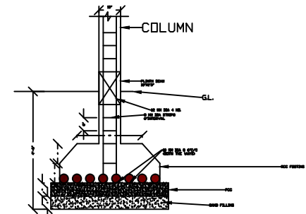
R.C.C. COLUMN DETAIL
