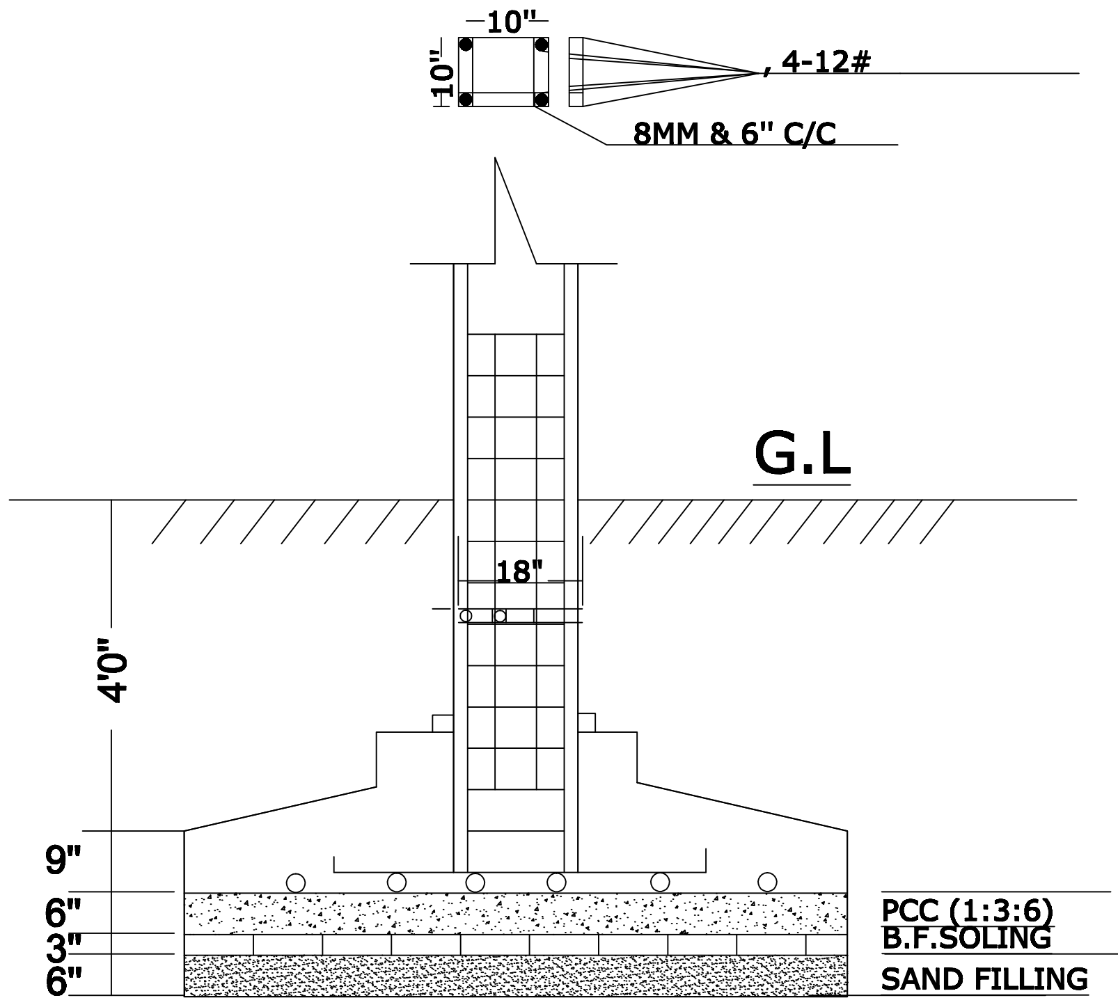
SECTION
