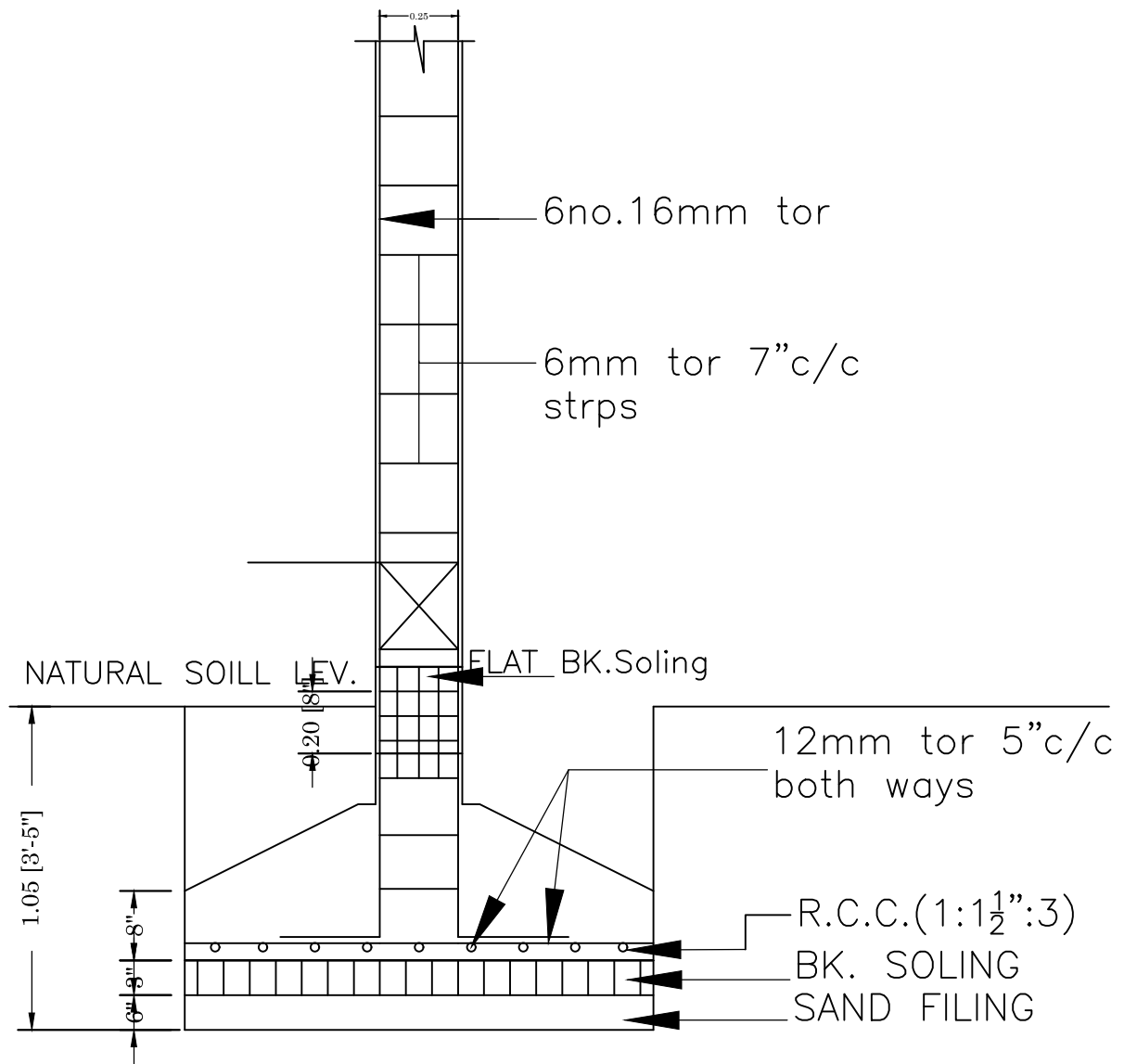
SEC. X-Y R.C.C. COLUMN FDN.DETAIL
