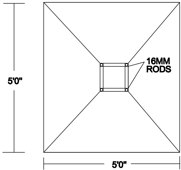
PLAN (SCALE 1"=4')
