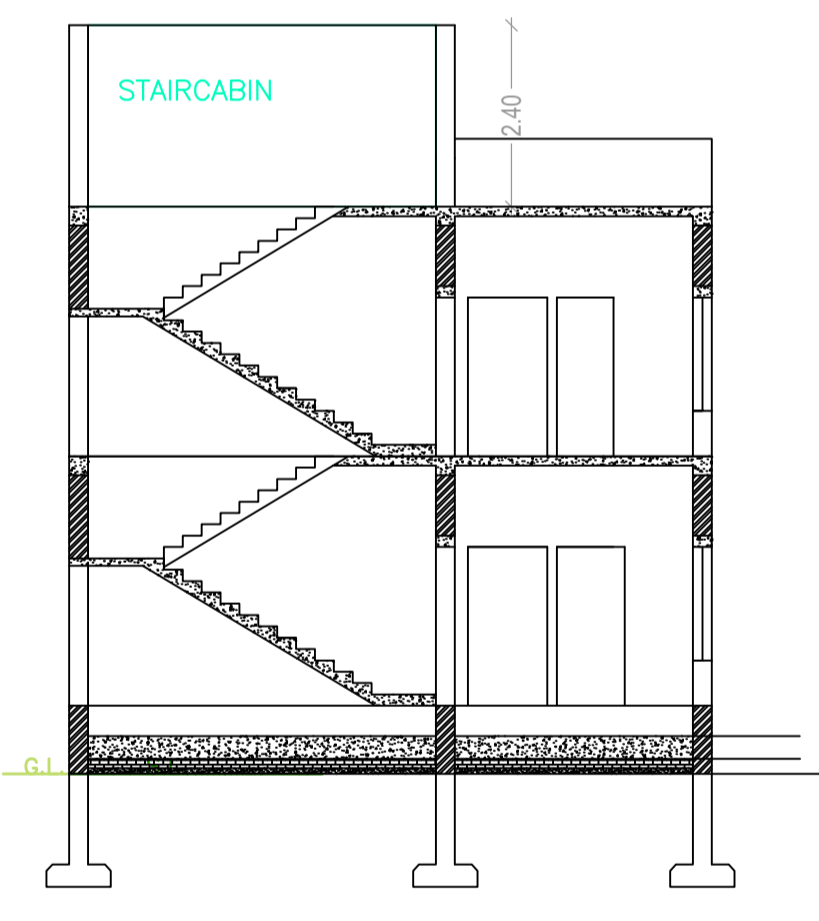
CROSS SECTION (A)
