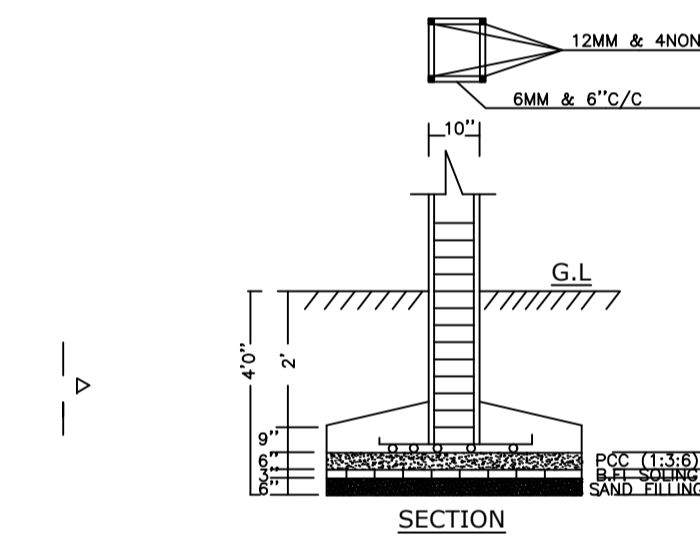
SECTION
